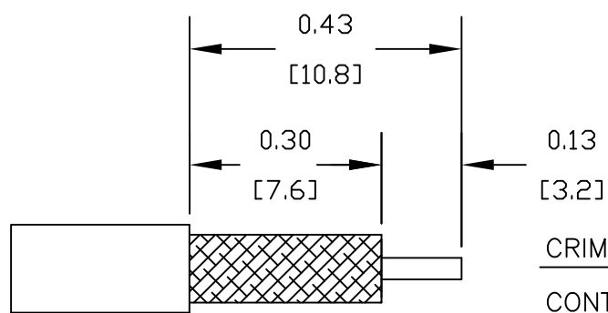
STRIPPING DIMENSIONS
