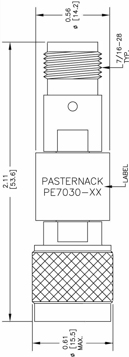
TNC FEMALE
