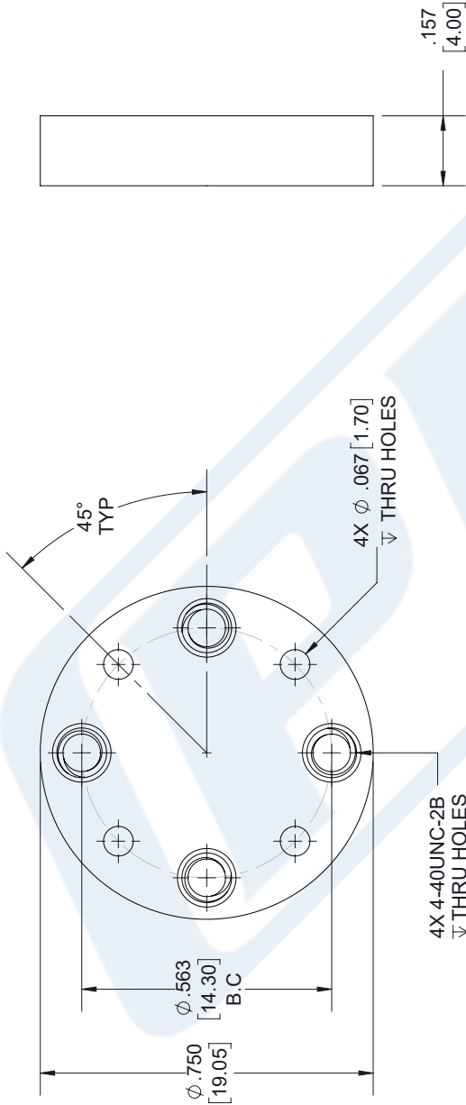
WR-15 WAVEGUIDE UG-385/U ROUND COVER FLANGE
