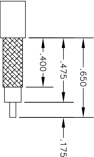
STRIPPING DIMENSIONS
