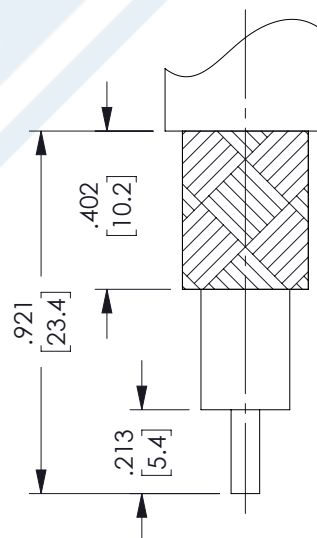
STRIPPING DIMENSIONS
