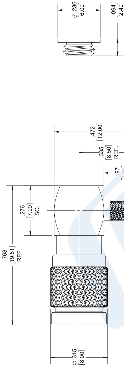
1.0/2.3 PLUG
