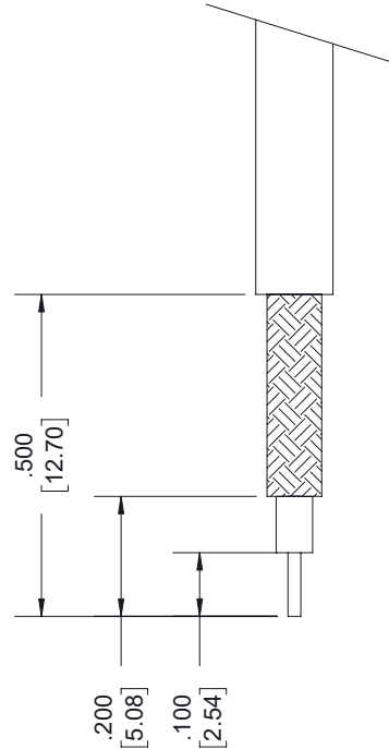
STRIPPING DIMENSIONS
