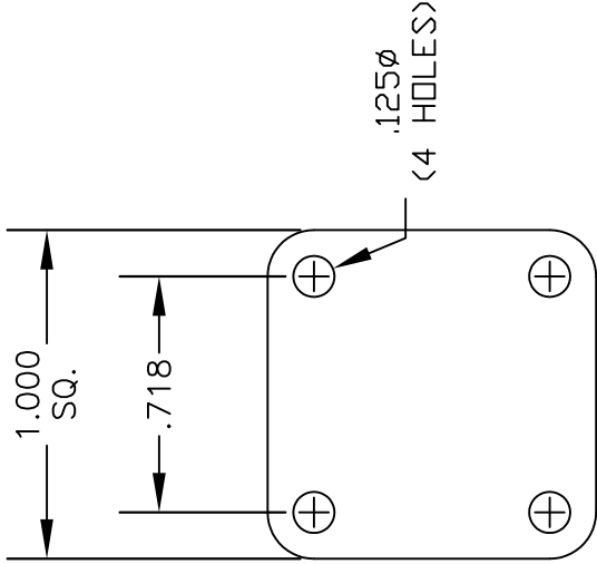
MOUNTING HOLES
