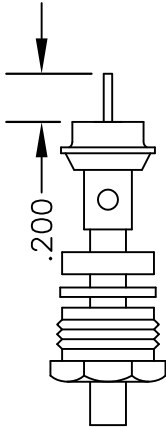
ASSEMBLY (B)
