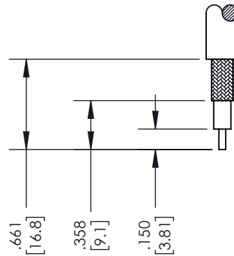
STRIPPING DIMENSIONS
