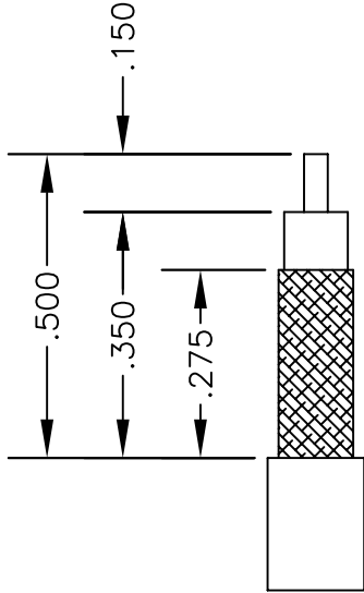
STRIPPING DIMENSIONS
