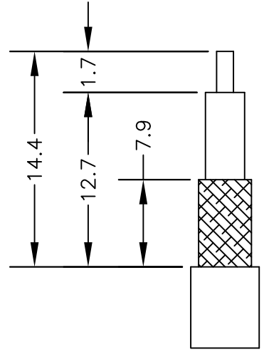
STRIPPING DIMENSIONS
